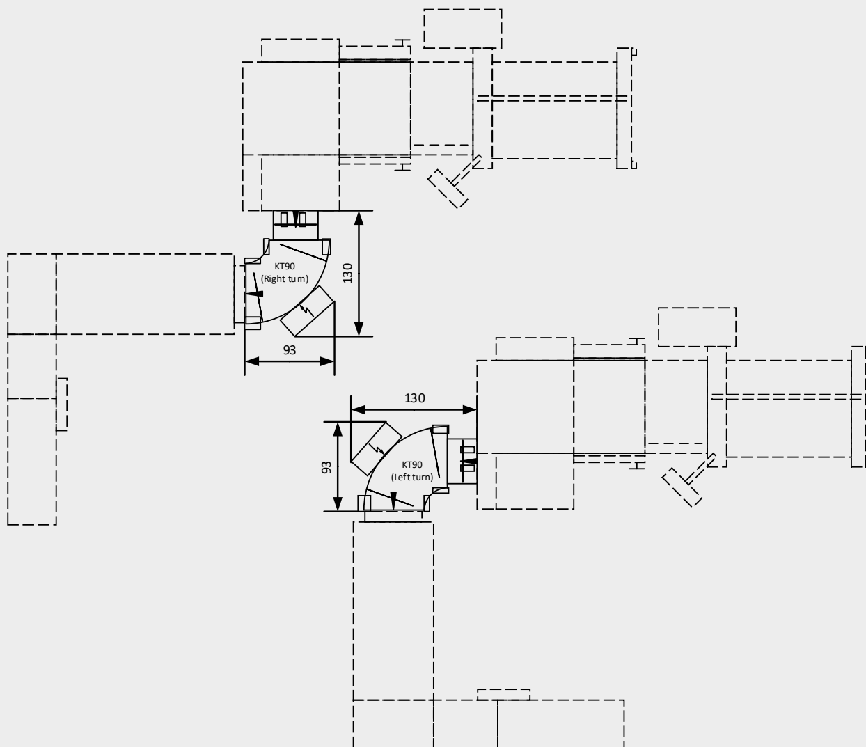
Floorplan KT90
