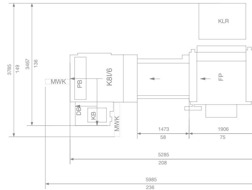
TECHNICAL DRAWING Floorplan K8i
