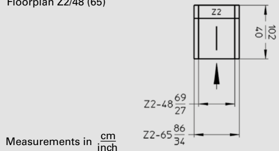
Floorplan Z2/48 (65)
